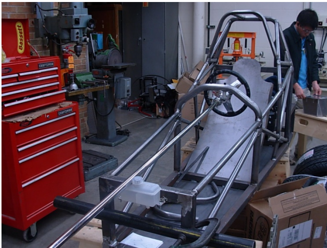
Chassis
